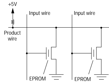
Figure 4. EPROM programmable switches.
