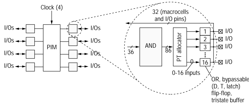
Figure 14. Cypress Flash370 architecture. (PIM: programmable interconnect matrix.)
