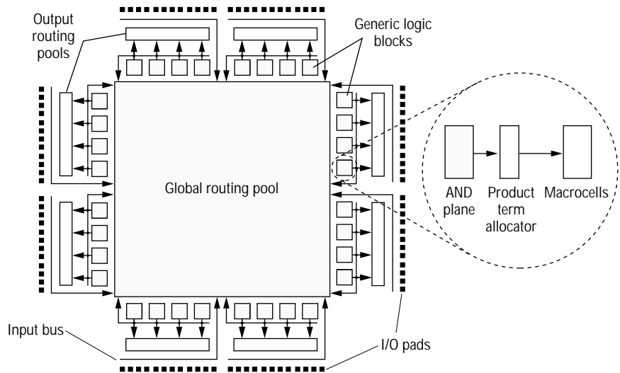
Figure 13. Lattice pLSI and ispLSI architecture.
