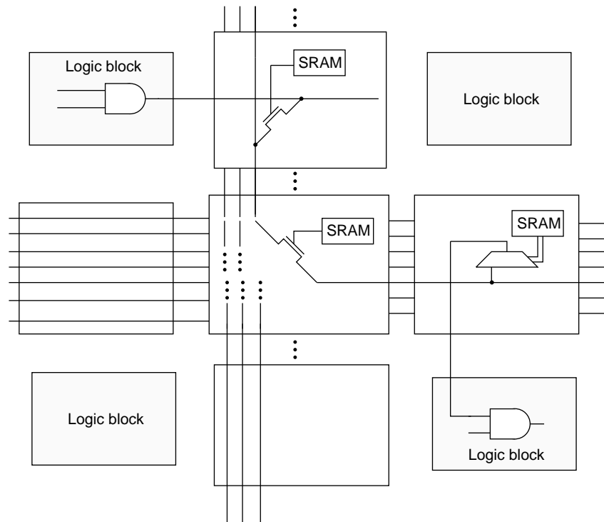
Figure 5. SRAM-controlled programmable switches.
