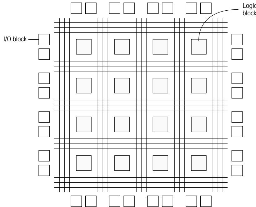
Figure 2. FPGA structure.
