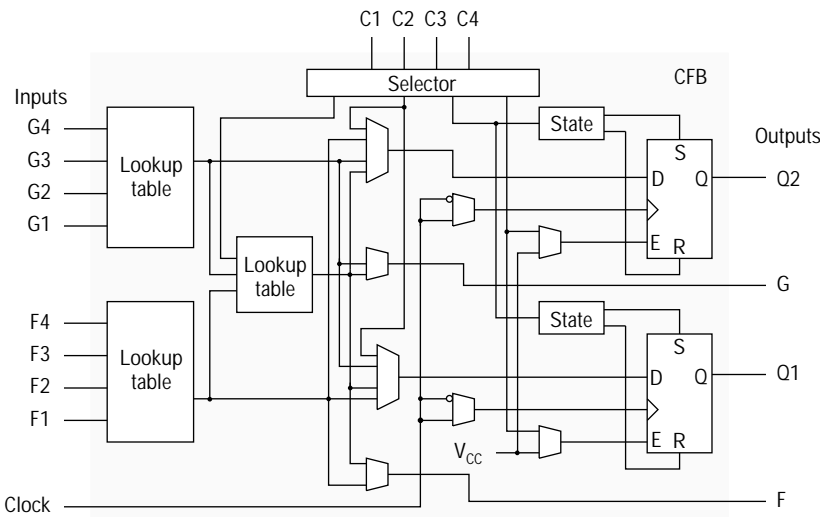
Figure 18. Xilinx XC4000 CLB.
