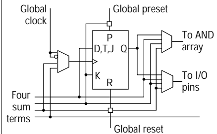
Figure 17. ICT PEEL Array logic cell structure.
